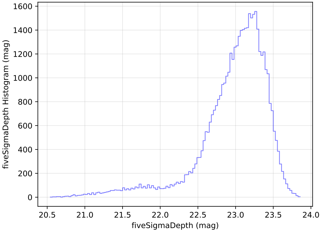
no_high_blob_v3.3_10yrs Yr 1 z band: fiveSigmaDepth Histogram
