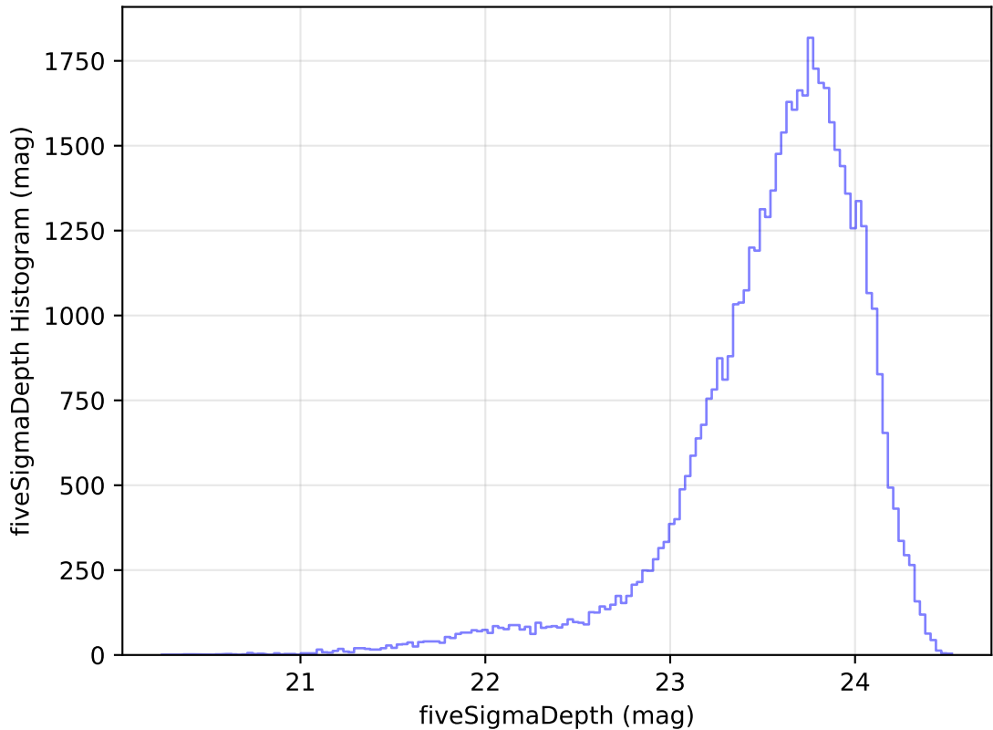
no_high_blob_v3.3_10yrs Yr 1 i band: fiveSigmaDepth Histogram
