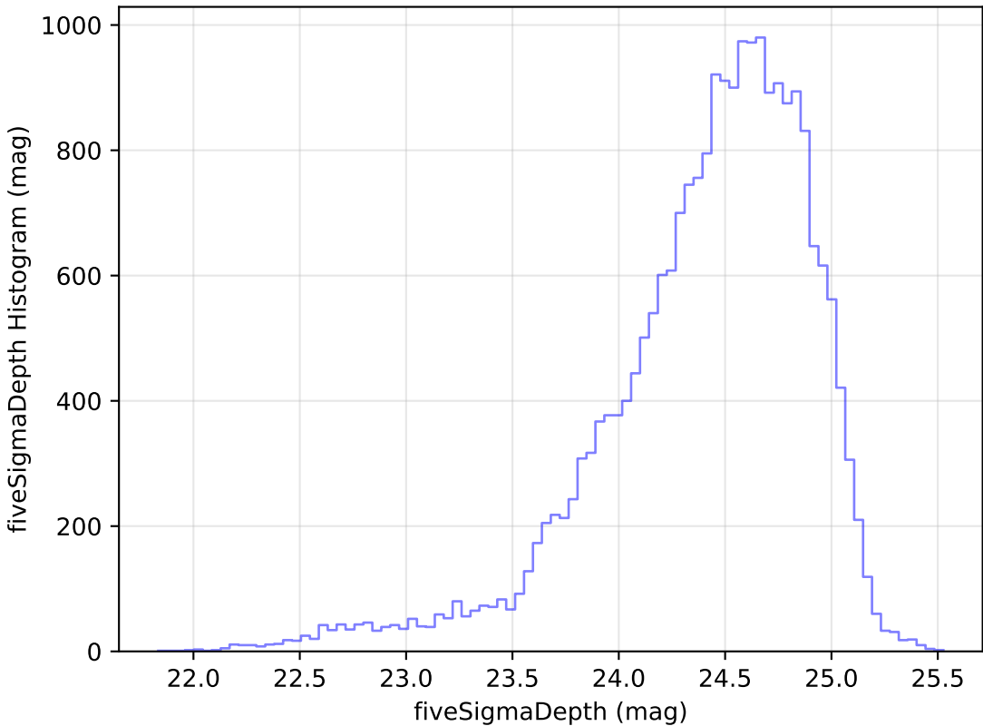
no_high_blob_v3.3_10yrs Yr 1 g band: fiveSigmaDepth Histogram
