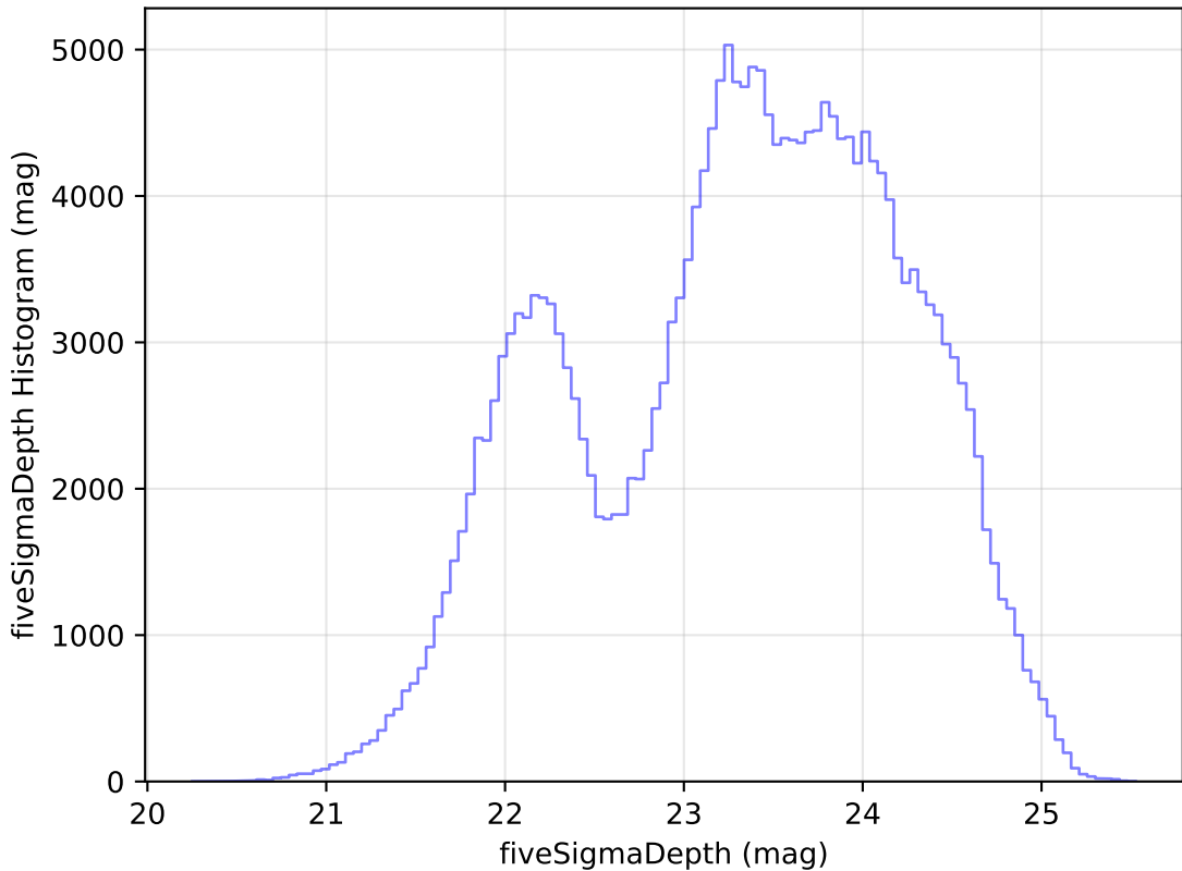
no_high_blob_v3.3_10yrs Yr 1 all bands: fiveSigmaDepth Histogram
