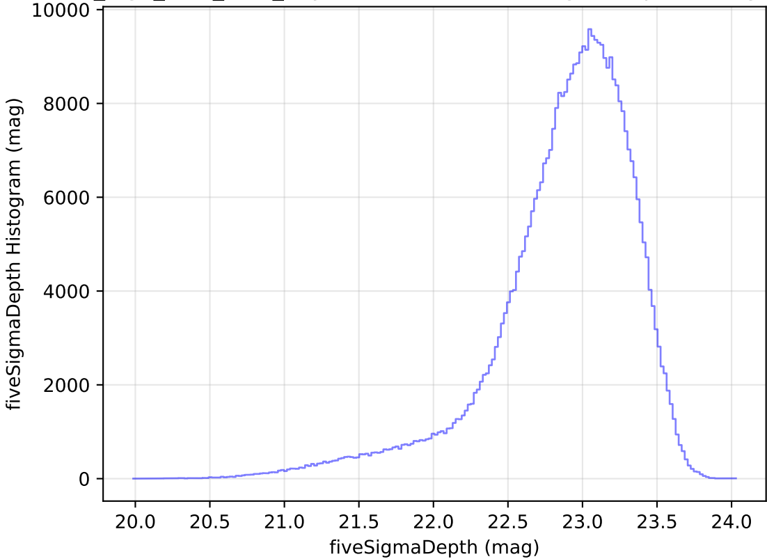
no_high_blob_v3.3_10yrs WFD z band: fiveSigmaDepth Histogram
