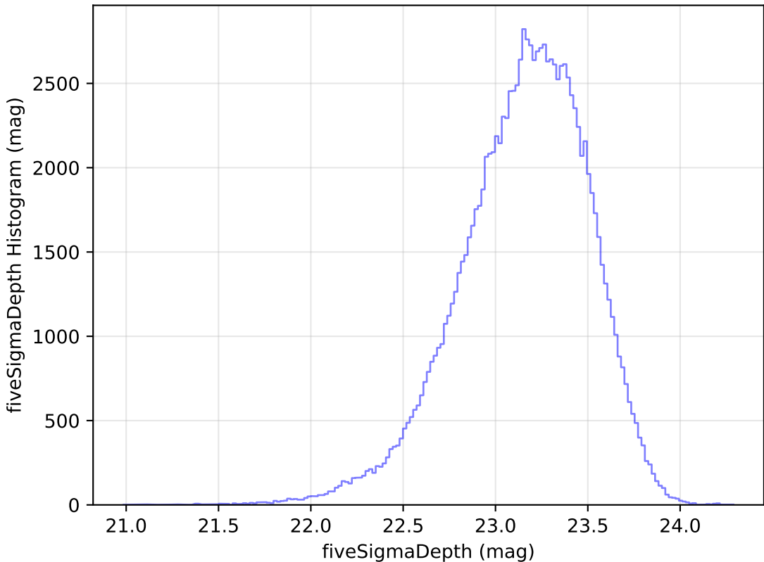
no_high_blob_v3.3_10yrs WFD u band: fiveSigmaDepth Histogram
