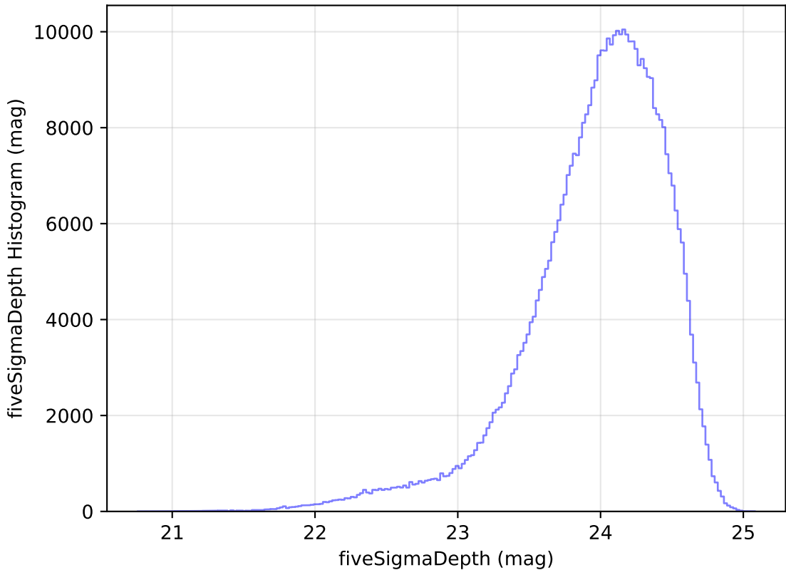
no_high_blob_v3.3_10yrs WFD r band: fiveSigmaDepth Histogram
