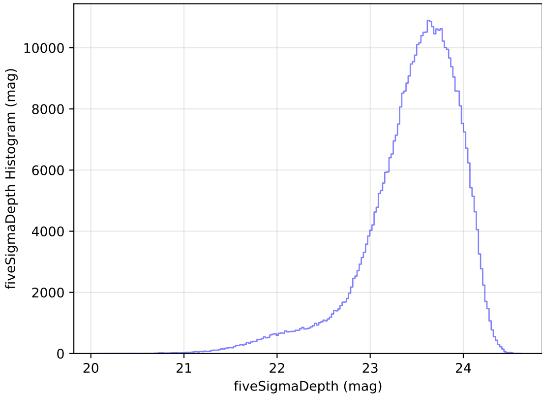
no_high_blob_v3.3_10yrs WFD i band: fiveSigmaDepth Histogram
