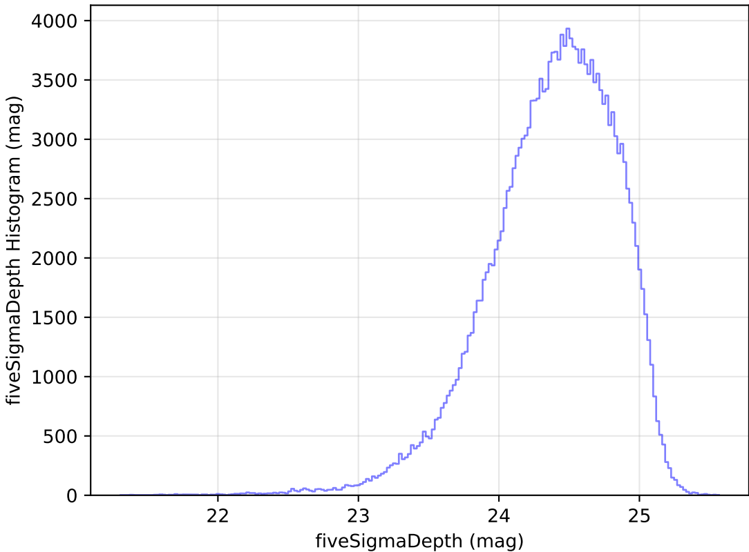
no_high_blob_v3.3_10yrs WFD g band: fiveSigmaDepth Histogram
