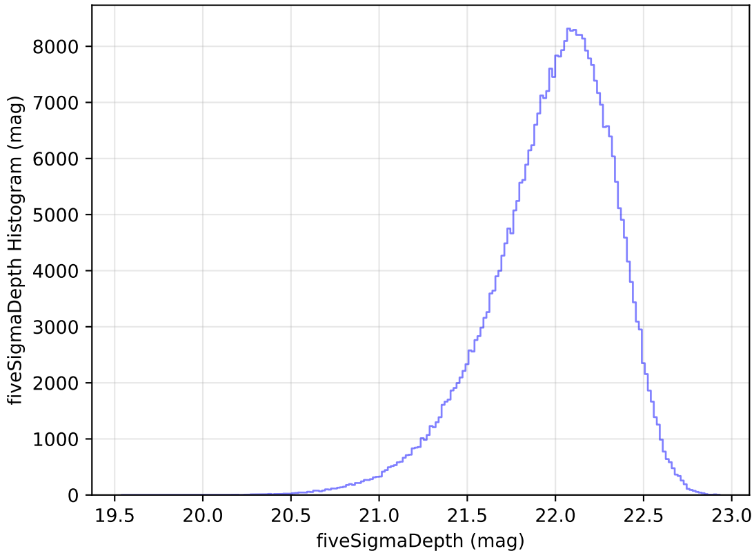
no_high_blob_v3.3_10yrs All sky y band: fiveSigmaDepth Histogram
