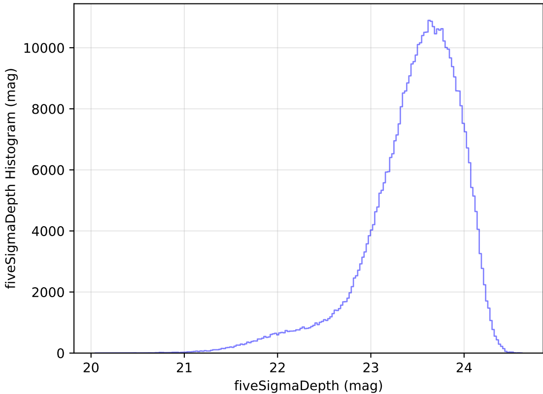
no_high_blob_v3.3_10yrs All sky i band: fiveSigmaDepth Histogram
