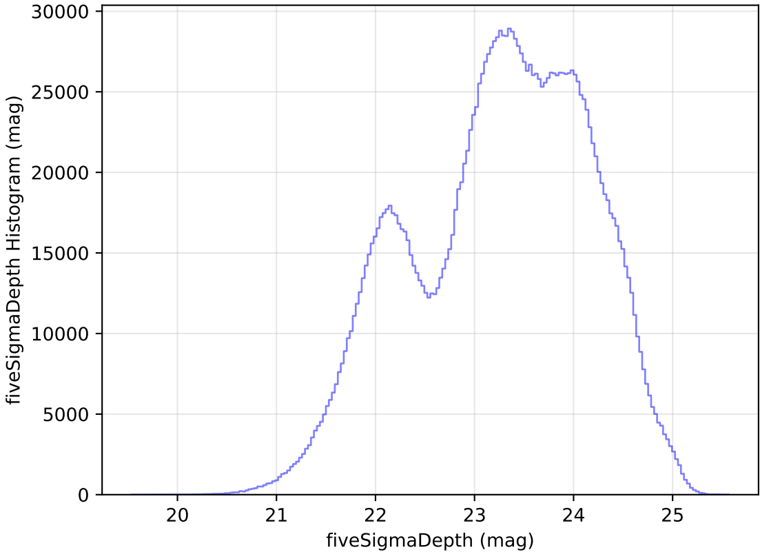
no_high_blob_v3.3_10yrs All sky all bands: fiveSigmaDepth Histogram
