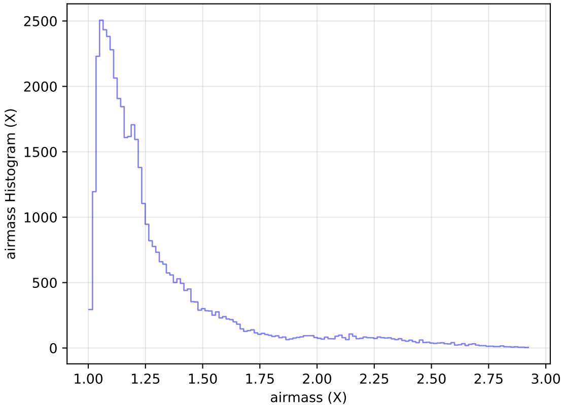
no_high_blob_v3.3_10yrs Yr 1 z band: airmass Histogram
