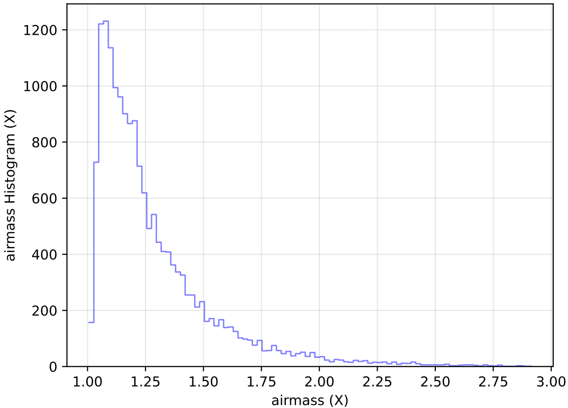
no_high_blob_v3.3_10yrs Yr 1 u band: airmass Histogram
