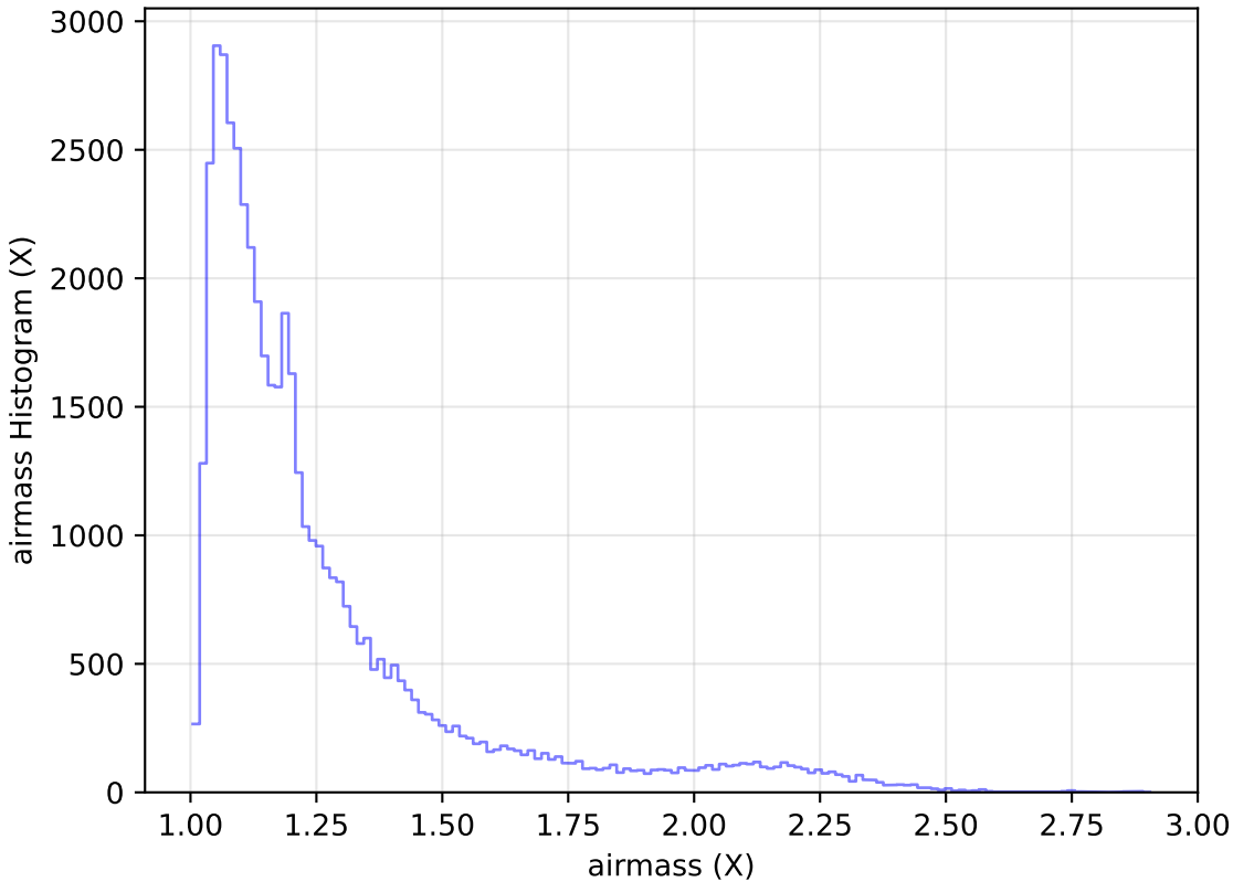
no_high_blob_v3.3_10yrs Yr 1 r band: airmass Histogram
