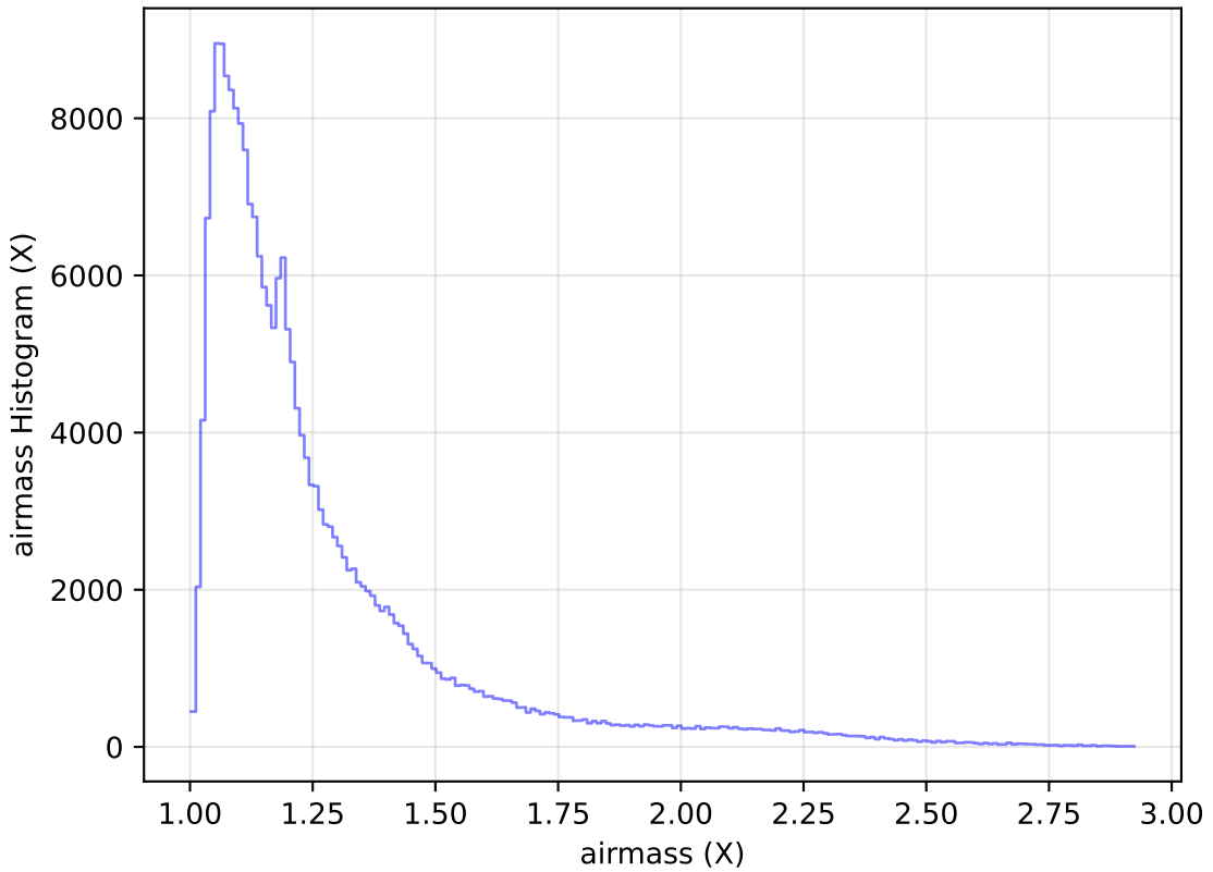
no_high_blob_v3.3_10yrs Yr 1 all bands: airmass Histogram
