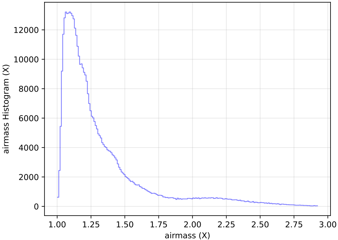
no_high_blob_v3.3_10yrs WFD z band: airmass Histogram
