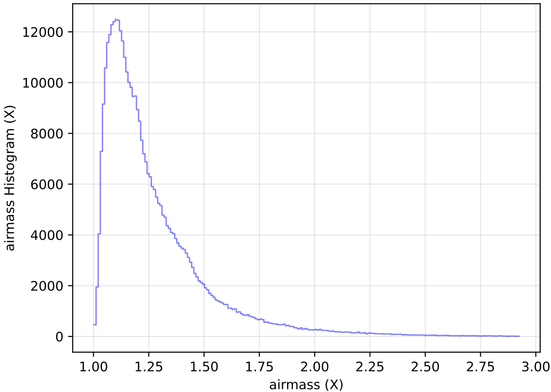
no_high_blob_v3.3_10yrs WFD y band: airmass Histogram
