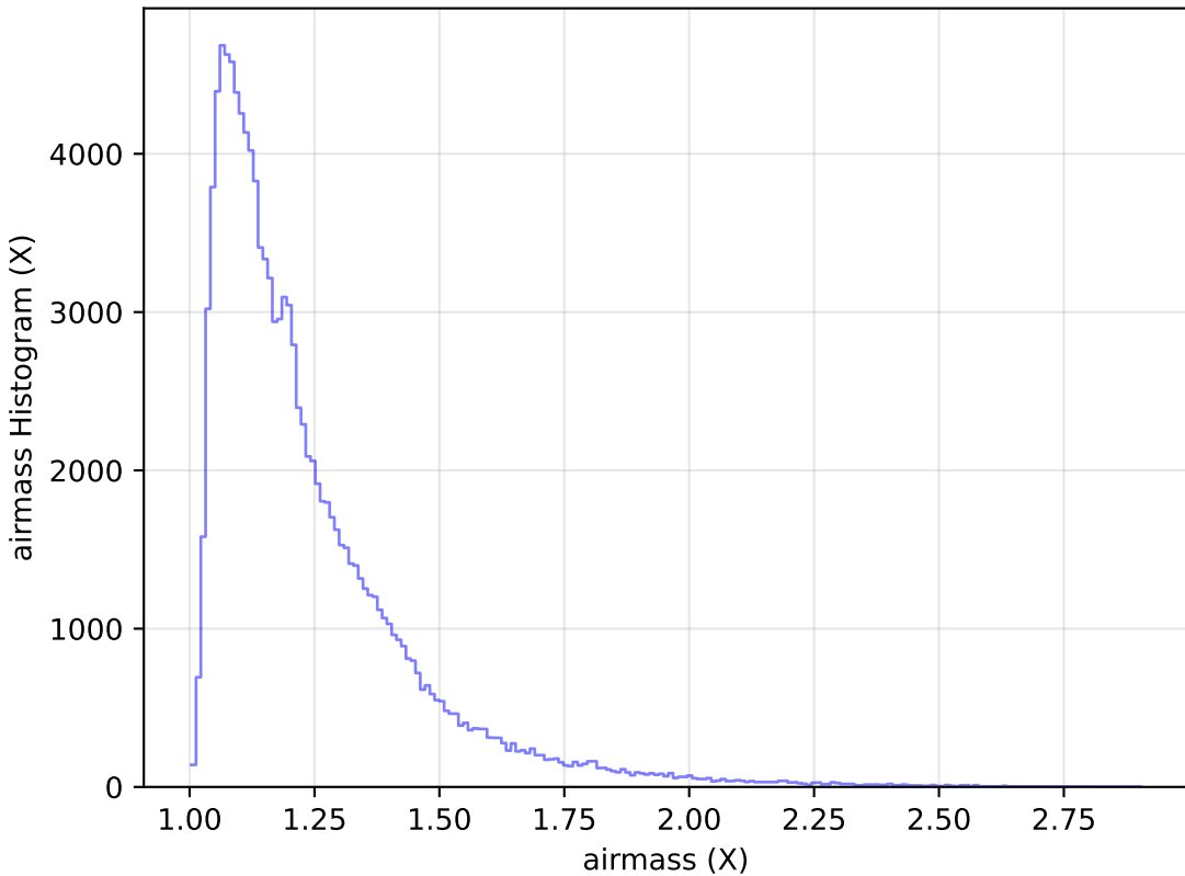
no_high_blob_v3.3_10yrs WFD u band: airmass Histogram
