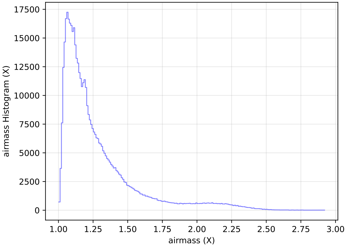
no_high_blob_v3.3_10yrs WFD r band: airmass Histogram
