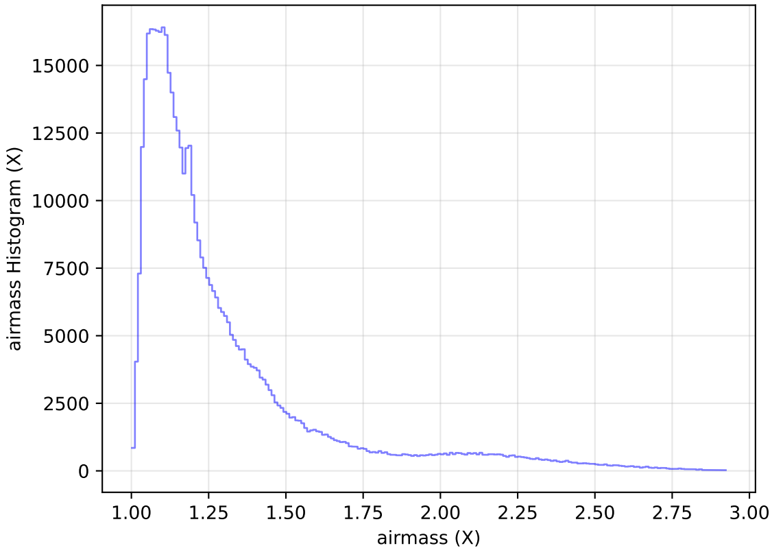
no_high_blob_v3.3_10yrs WFD i band: airmass Histogram
