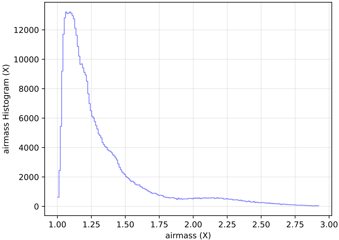
no_high_blob_v3.3_10yrs All sky z band: airmass Histogram
