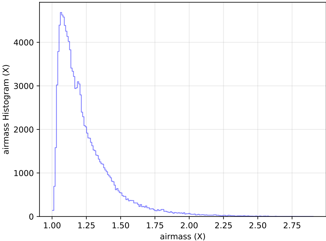
no_high_blob_v3.3_10yrs All sky u band: airmass Histogram
