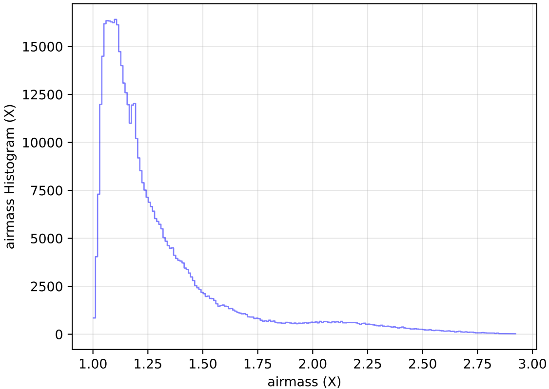
no_high_blob_v3.3_10yrs All sky i band: airmass Histogram
