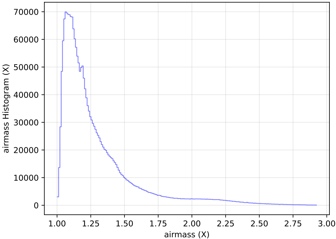
no_high_blob_v3.3_10yrs All sky all bands: airmass Histogram
