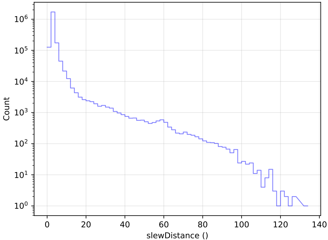
no_high_blob_v3.3_10yrs All visits: Slew Distance Histogram
