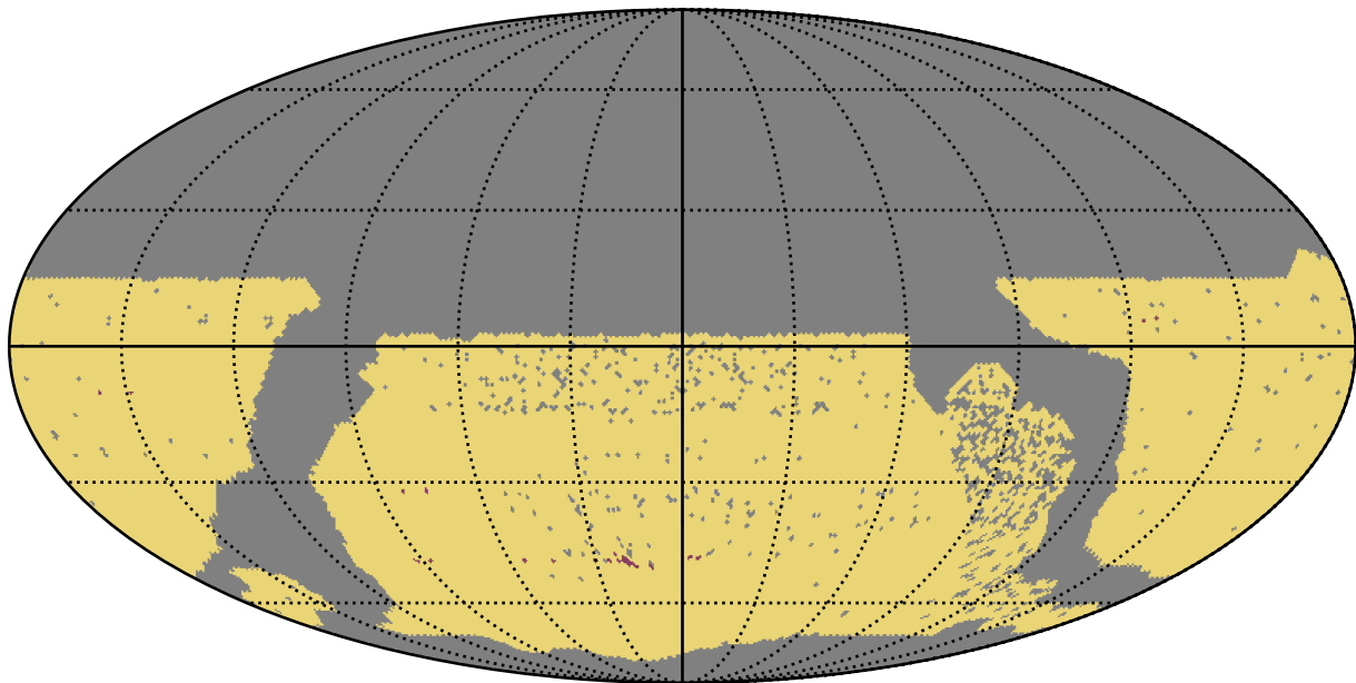
no_high_blob_v3.3_10yrs WFD: RapidRevisits
