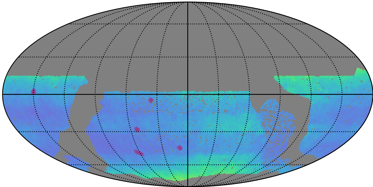
no_high_blob_v3.3_10yrs WFD: Proper Motion Uncert @ 24.0
