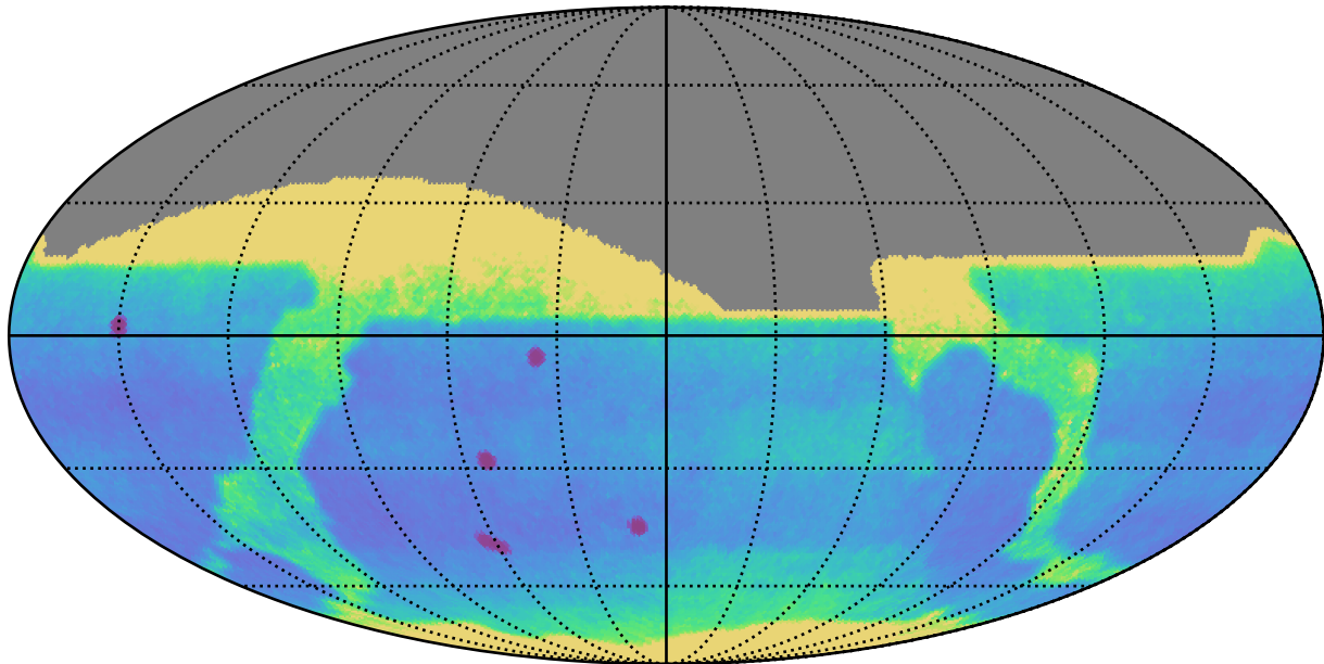
no_high_blob_v3.3_10yrs All sky: Proper Motion Uncert @ 24.0
