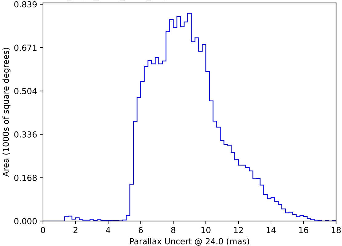
no_high_blob_v3.3_10yrs WFD: Parallax Uncert @ 24.0
