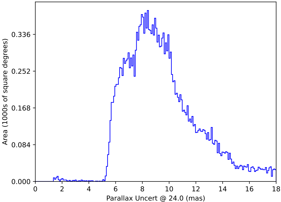
no_high_blob_v3.3_10yrs All sky: Parallax Uncert @ 24.0
