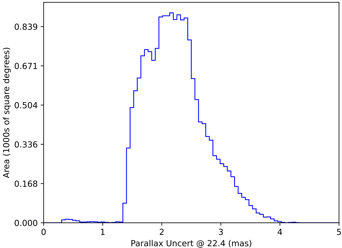
no_high_blob_v3.3_10yrs WFD: Parallax Uncert @ 22.4
