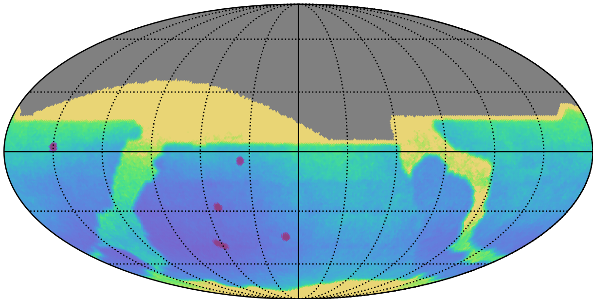
no_high_blob_v3.3_10yrs All sky: Parallax Uncert @ 22.4
