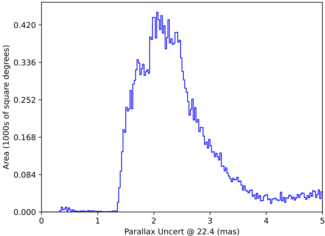
no_high_blob_v3.3_10yrs All sky: Parallax Uncert @ 22.4
