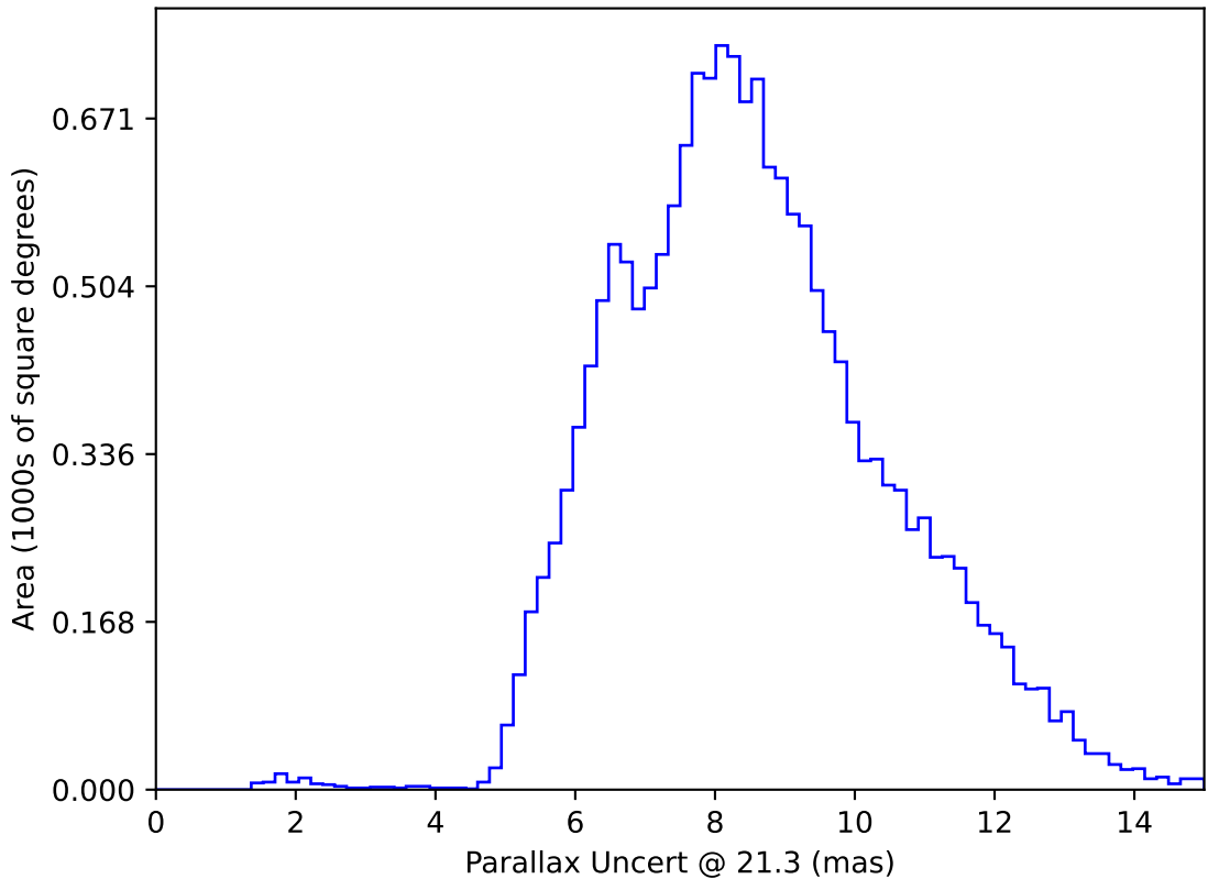
no_high_blob_v3.3_10yrs WFD y band only: Parallax Uncert @ 21.3
