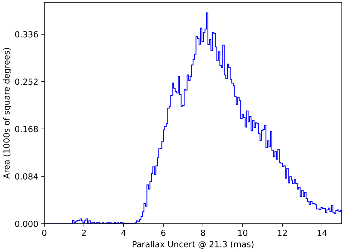
no_high_blob_v3.3_10yrs All sky y band only: Parallax Uncert @ 21.3
