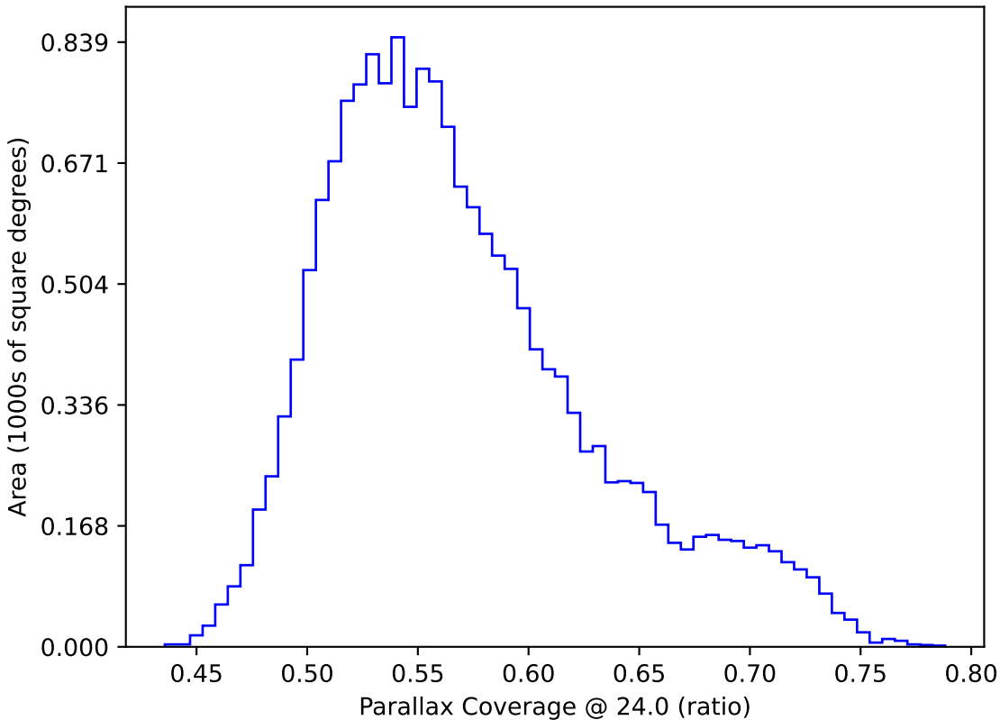
no_high_blob_v3.3_10yrs WFD: Parallax Coverage @ 24.0
