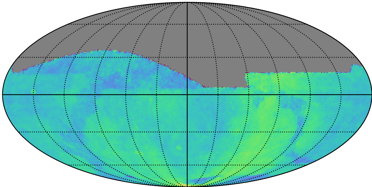
no_high_blob_v3.3_10yrs All sky: Parallax Coverage @ 24.0
