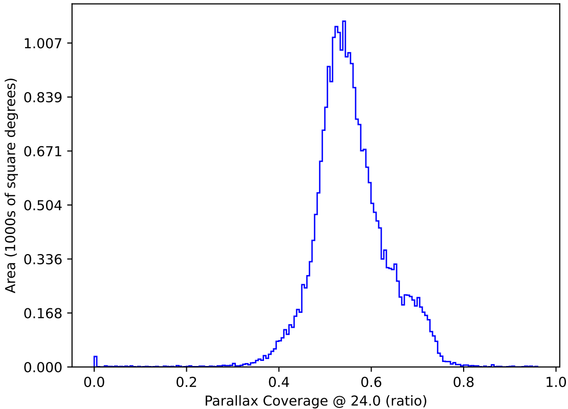
no_high_blob_v3.3_10yrs All sky: Parallax Coverage @ 24.0
