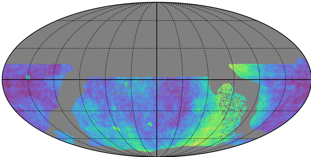
no_high_blob_v3.3_10yrs WFD: Parallax Coverage @ 22.4
