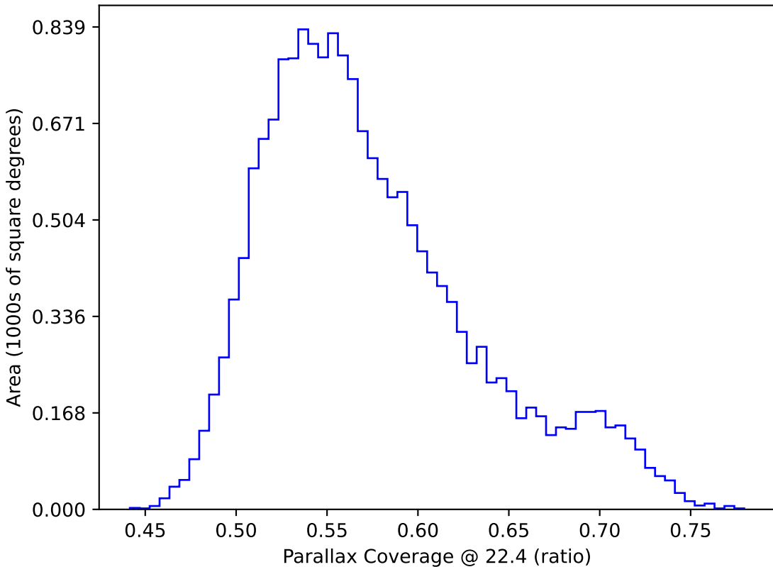
no_high_blob_v3.3_10yrs WFD: Parallax Coverage @ 22.4
