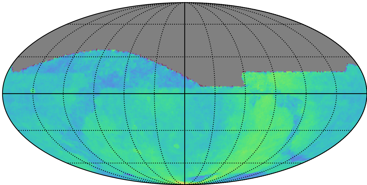
no_high_blob_v3.3_10yrs All sky: Parallax Coverage @ 22.4
