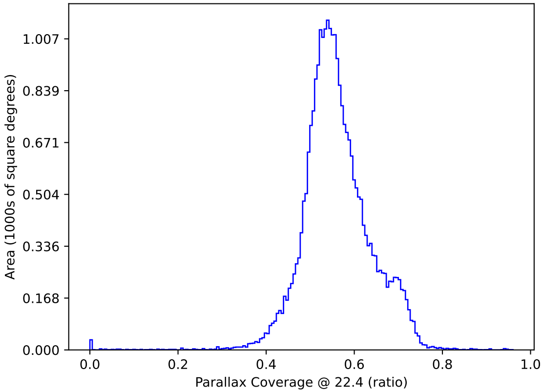
no_high_blob_v3.3_10yrs All sky: Parallax Coverage @ 22.4
