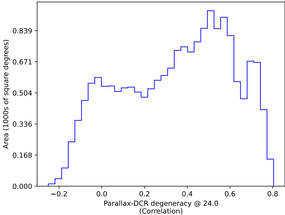
no_high_blob_v3.3_10yrs WFD: Parallax-DCR degeneracy @ 24.0
