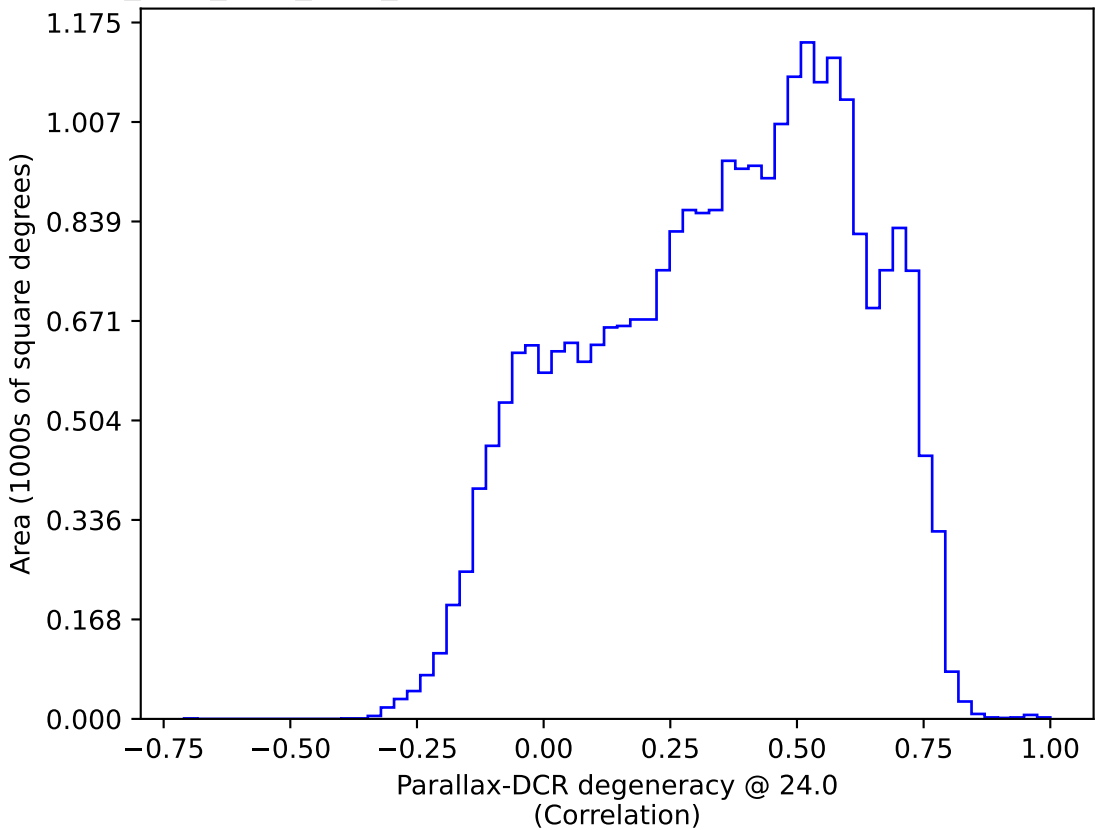
no_high_blob_v3.3_10yrs All sky: Parallax-DCR degeneracy @ 24.0
