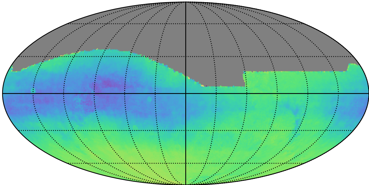
no_high_blob_v3.3_10yrs All sky: Parallax-DCR degeneracy @ 22.4
