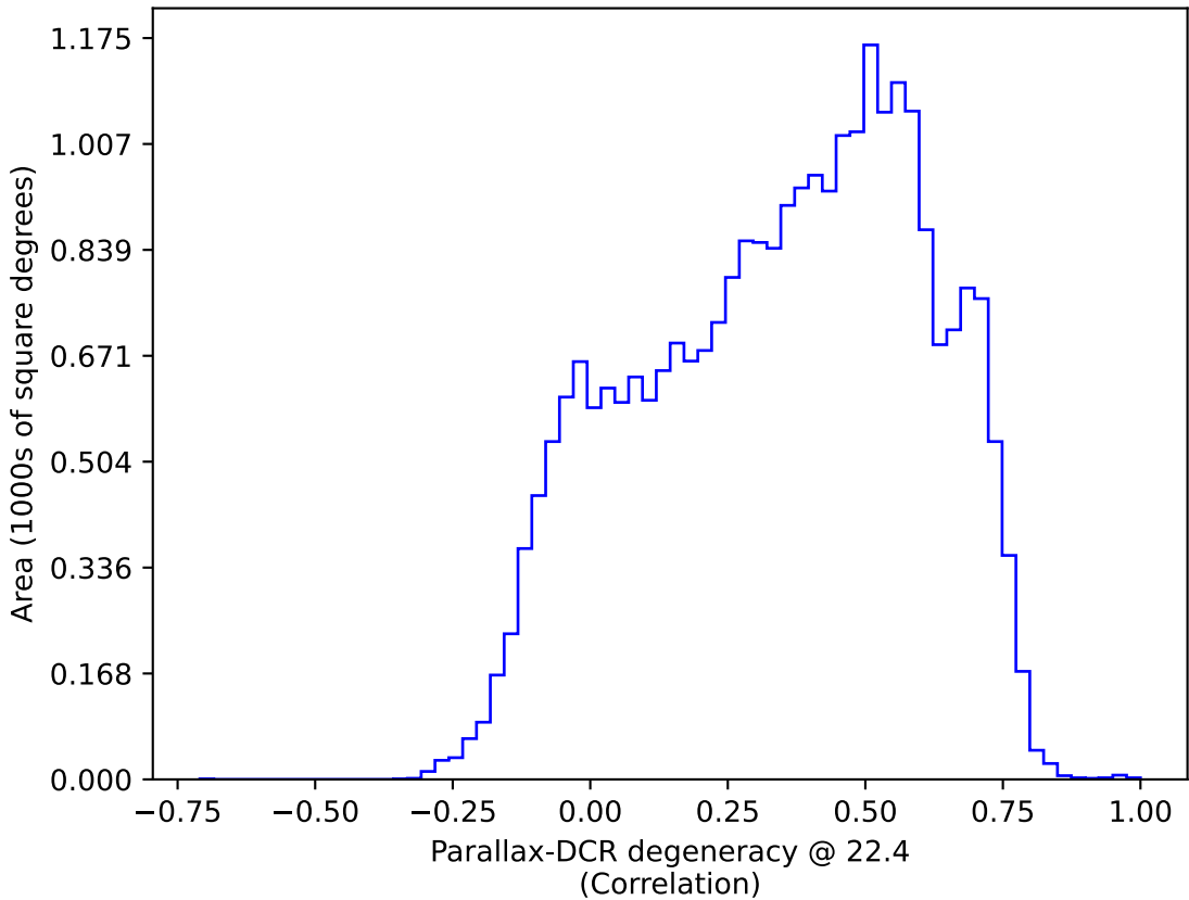
no_high_blob_v3.3_10yrs All sky: Parallax-DCR degeneracy @ 22.4
