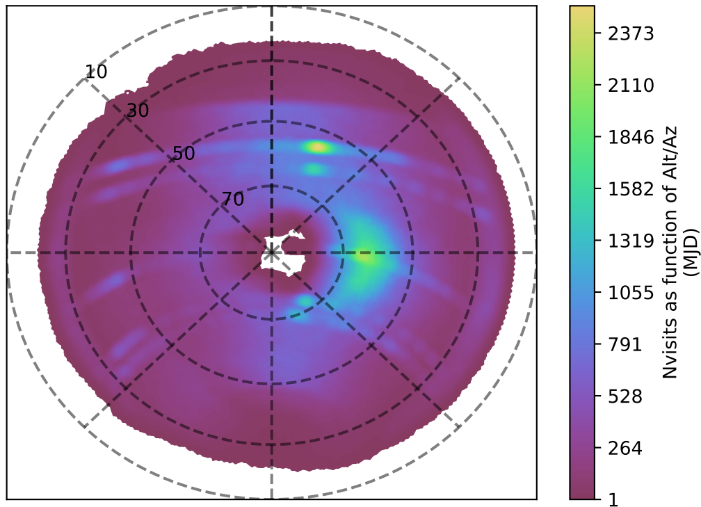
no_high_blob_v3.3_10yrs z band: Nvisits as function of Alt/Az
