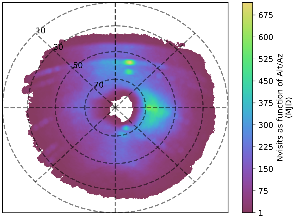
no_high_blob_v3.3_10yrs u band: Nvisits as function of Alt/Az
