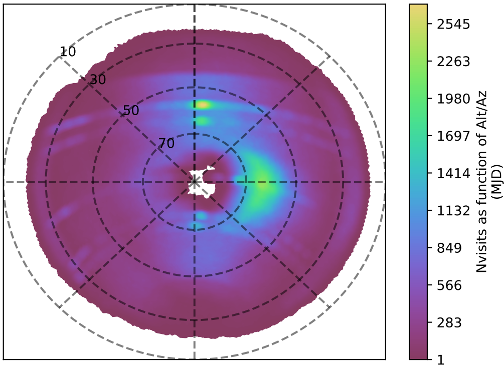
no_high_blob_v3.3_10yrs i band: Nvisits as function of Alt/Az
